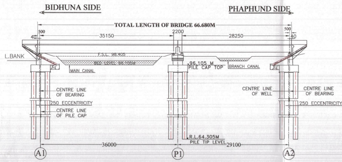
SECTIONAL ELEVATION OF BRIDGE
