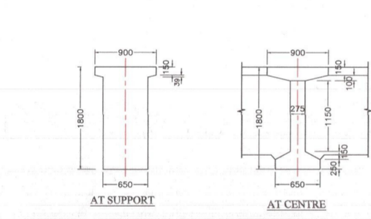
X- SEC. OF P.S.C. BEAM FOR 28.25M C/C OF BEARING
