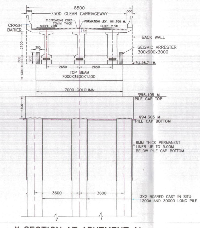
X-SECTION AT ABUTMENT A1
