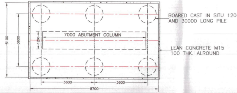
TYP. PLAN AT PILE CAP
