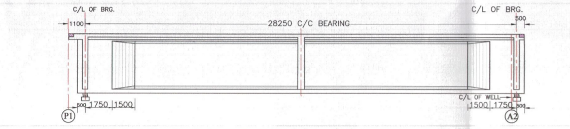
SECTIONAL ELEVATION OF P.S.C. GIRDER OF 28.250M C/C OF BEARING
