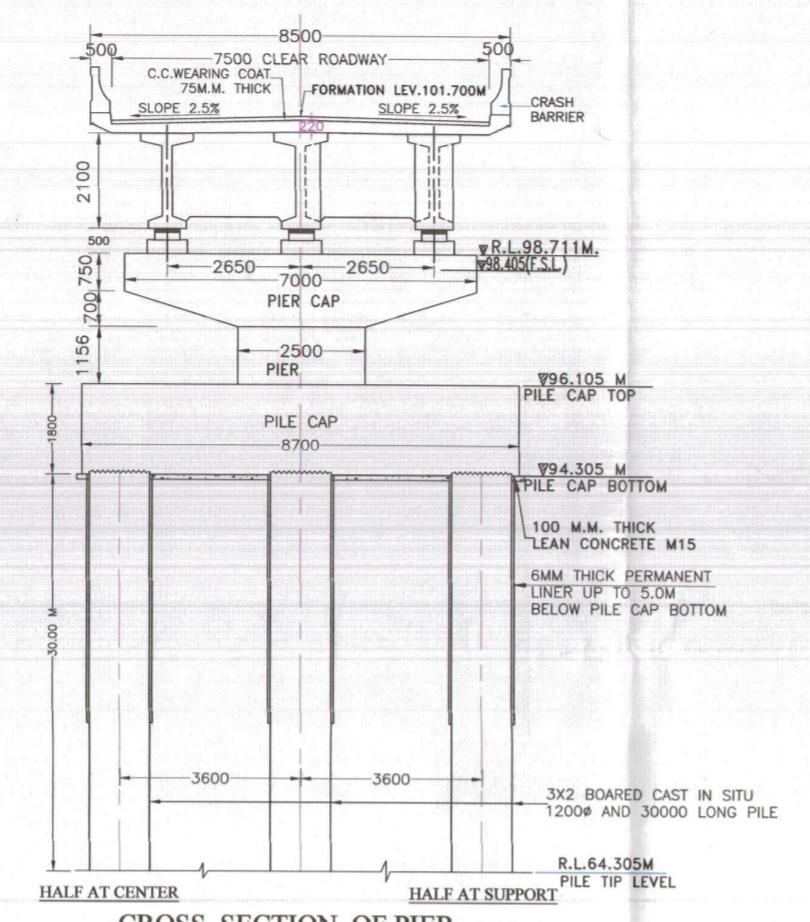
CROSS SECTION OF PIER
