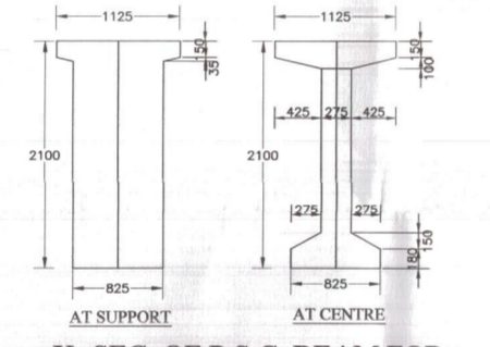
X- SEC. OF P.S.C. BEAM FOR 35.150M C/C OF BEARING
