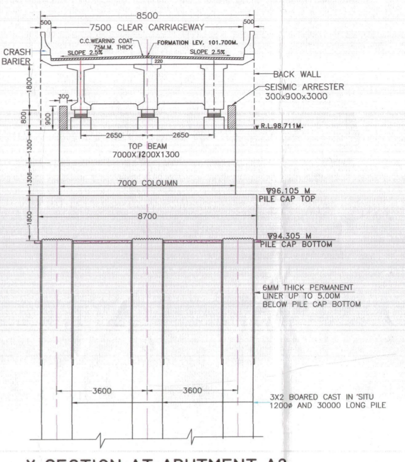
X-SECTION AT ABUTMENT A2
