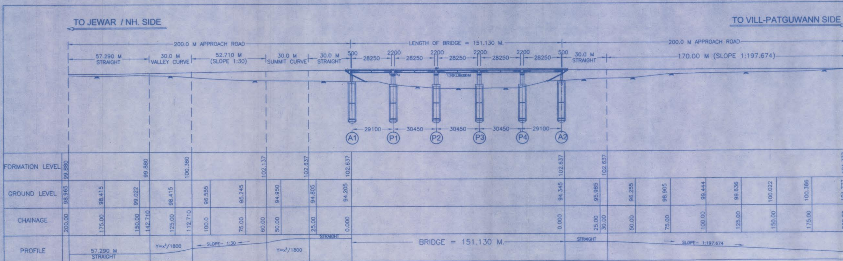
GENERAL ELEVATION OF BRIDGE & APPROACH ROAD
