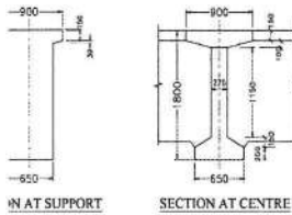
CROSS SECTION OF P.S.C. BEAM
