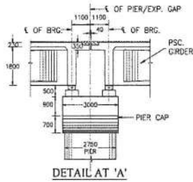
DETAIL AT 'A'
