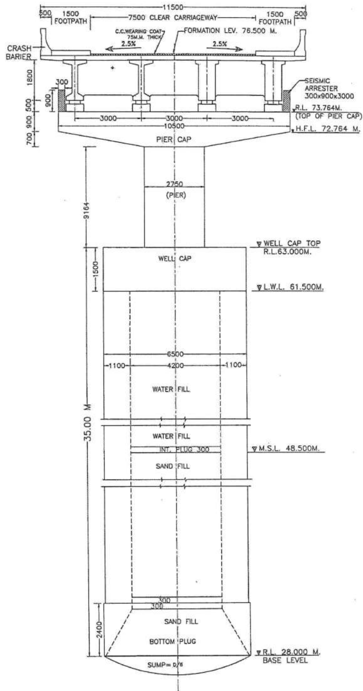
HALF AT CENTRE HALF AT SUPPORT CROSS - SECTION
