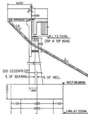
CROSS SECTION AT ABUTMENT
