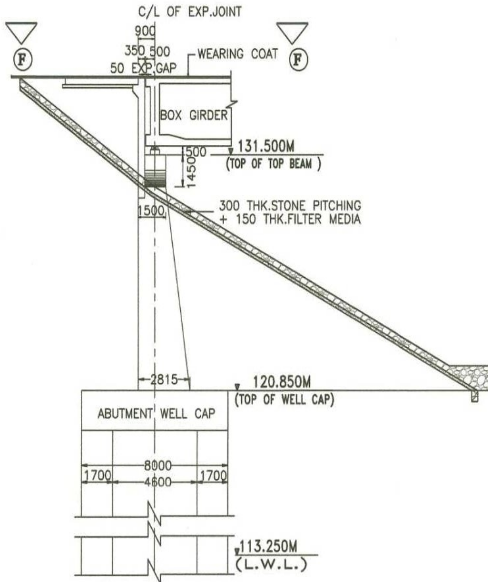
TYPICAL CROSS SECTION OF ABUTMENT
