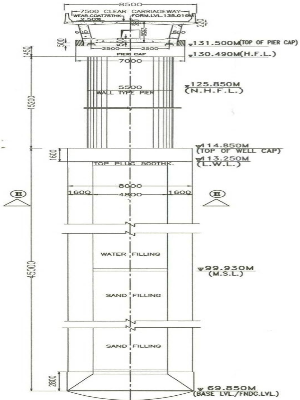
TYPICAL CROSS SECTION OF PIER
