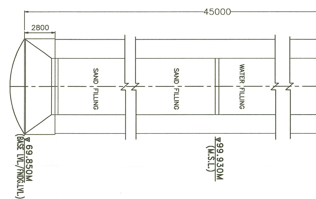
TYPICAL CROSS SECTION OF PIER
