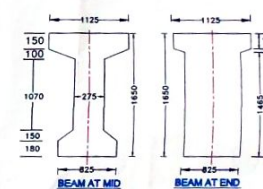
X-SEC. OF P.S.C.BEAM FOR 25.500M SAN (P16-P17 SPAN)
