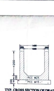
TYP. CROSS SECTION OF DRAIN
