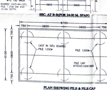
PLAN SHOWING PILE & PILE CAP
