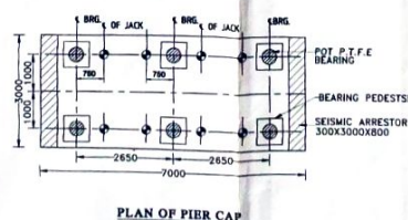
PLAN OF PIER CAP
