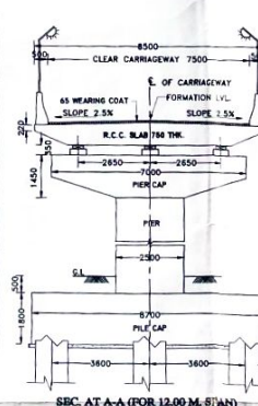
SEC. AT A-A (FOR 12.00 M. SPAN)
