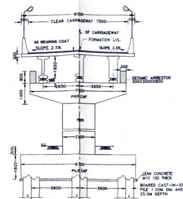
SEC. AT C-C(FOR 25.560 M. SPAN) (P16-P17 SPAN)
