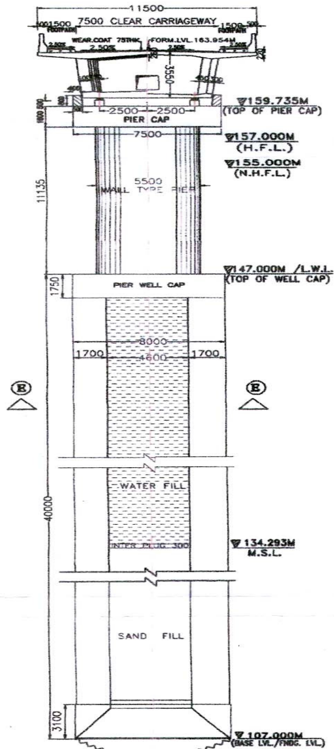
TYP. CROSS SEC. OF PIER FOR 58.50M PIER SPAN
