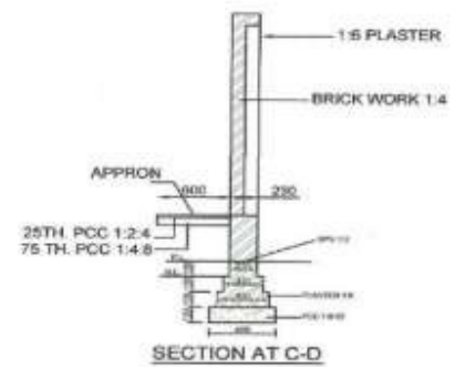
SECTION AT C-D
