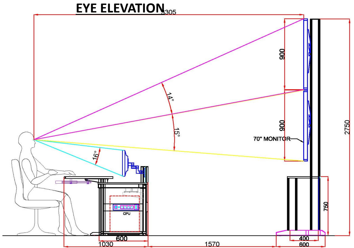
MONITOR WALL AS PER SITE REQUIRED MATRIX
