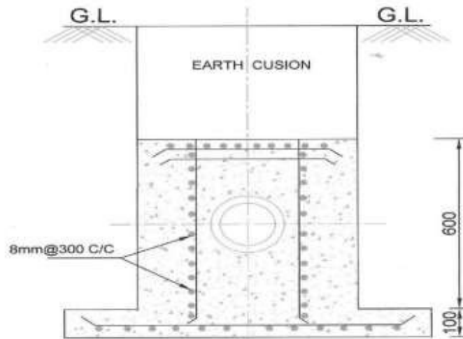
SECTION AT A-A'
