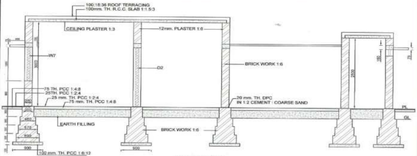
SECTION AT A-B
