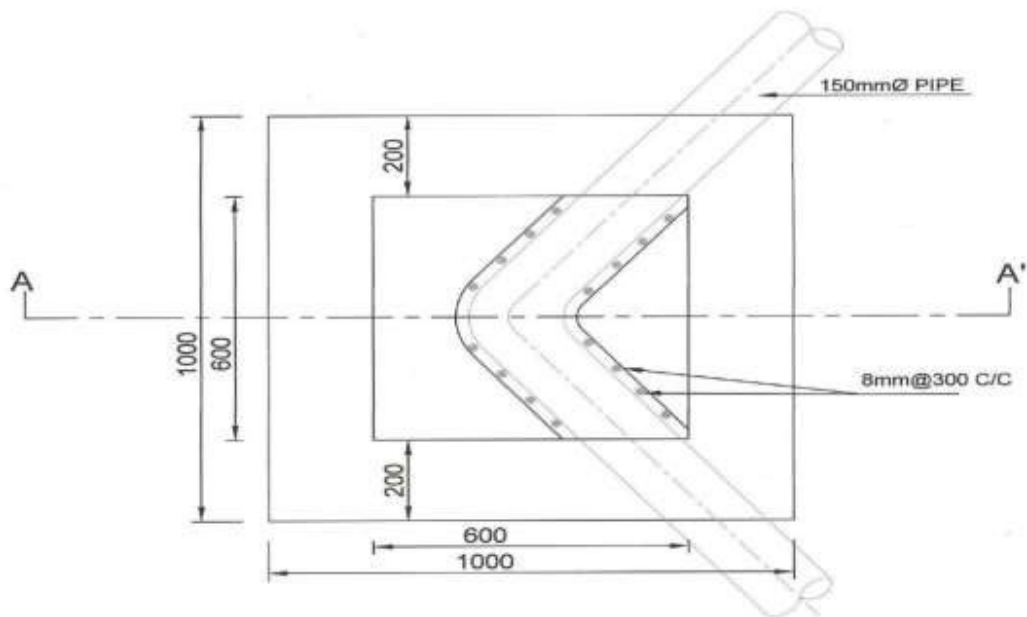
PLAN
