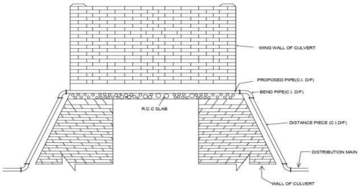
ELEVATION AT X-Y
