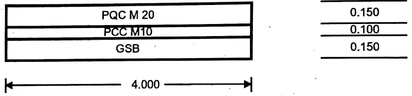
TYPICAL CROSS SECTION PCC ROAD
