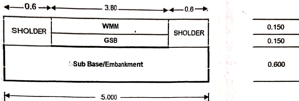
TYPICAL CROSS SECTION WBM ROAD
