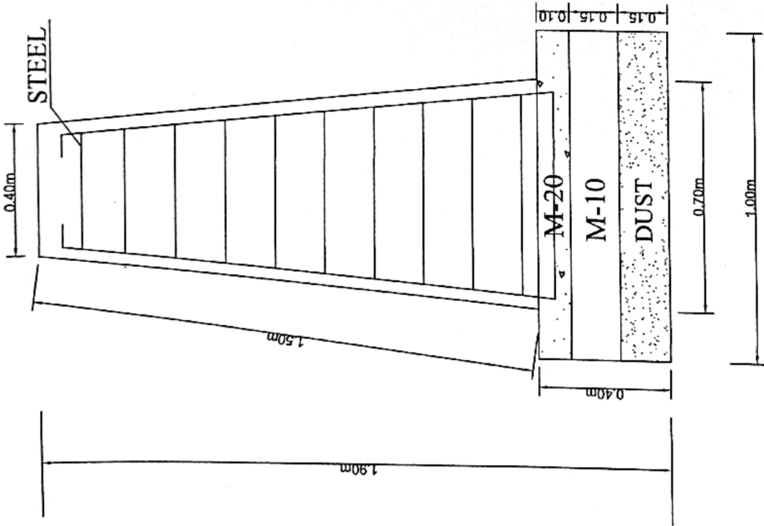
C/S OF RETAINING WALL
