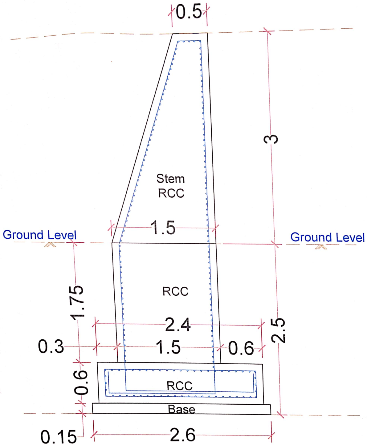
C/s of Retaining Wall
