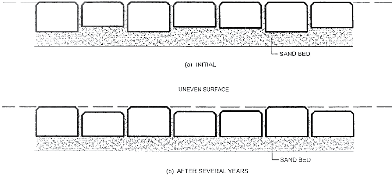
Fig. 7 Effect of Thickness Variations in Paving Blocks
