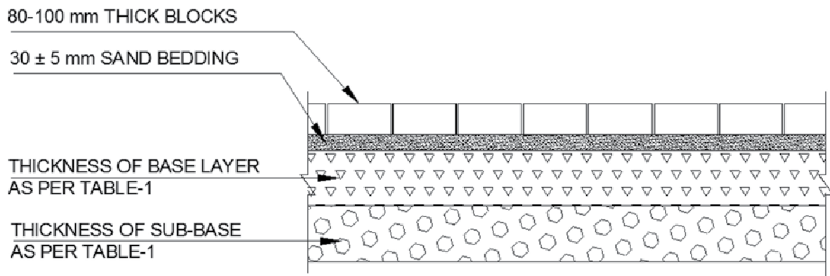
Fig.6A Typical Cross Section of Block Pavement for Medium and Heavily Trafficked Road except National-Highways, Expressways, State Highways and MDR
