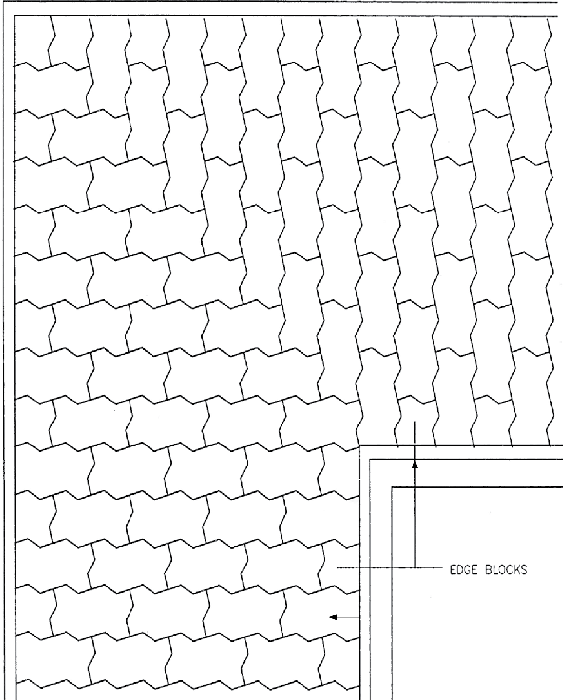
Fig.2190° Change in Alignment using Stretcher Bond
