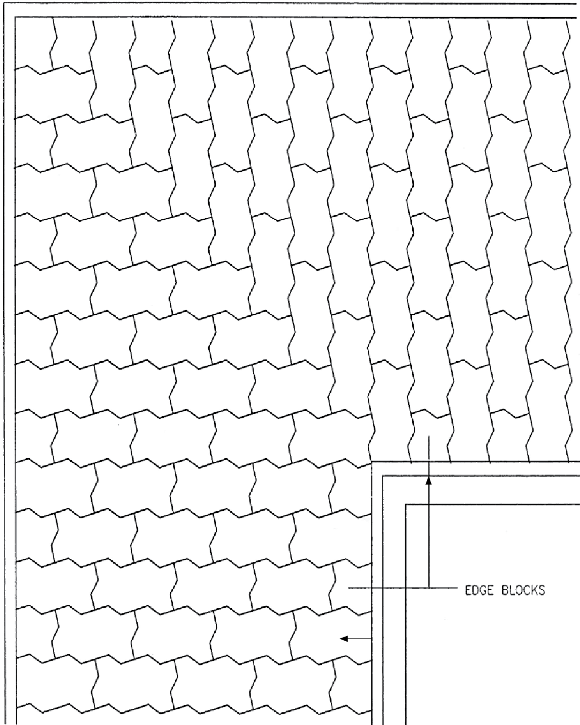
Fig.2 190° Change in Alignment using Stretcher Bond
