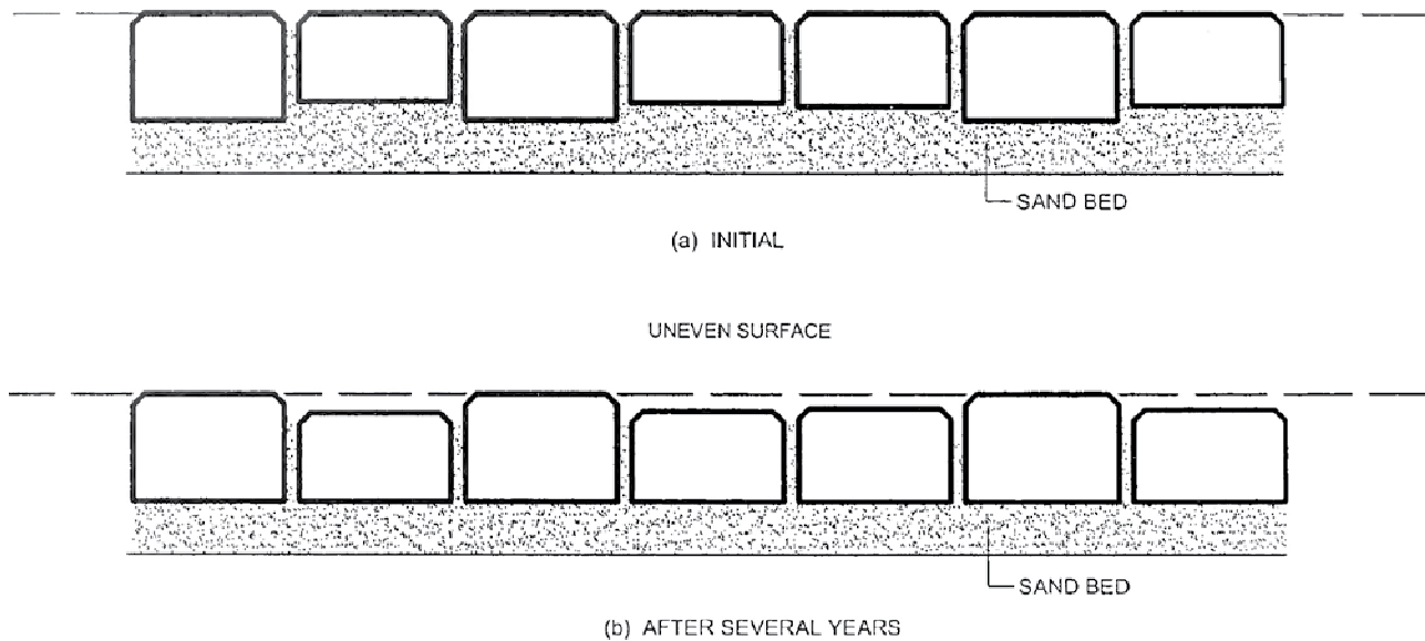
Fig.7EffectofThicknessVariationsinPavingBlocks
