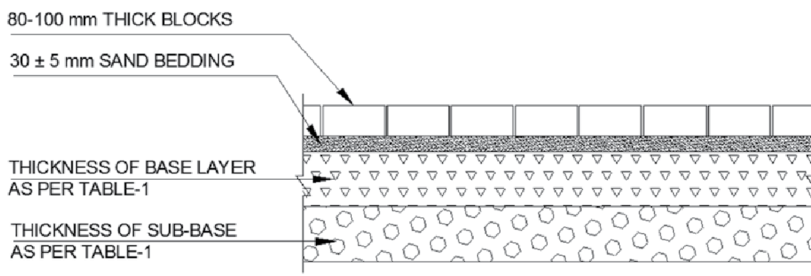
Fig. 6 Typical Cross Section of Block Pavement for Medium and Heavily Trafficked Roads except National-Highways, Expressways, State Highways and MDR
