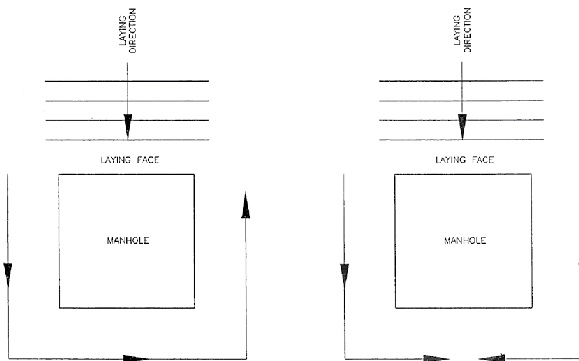
Fig.20.LayingBlockPavingAroundaManhole
