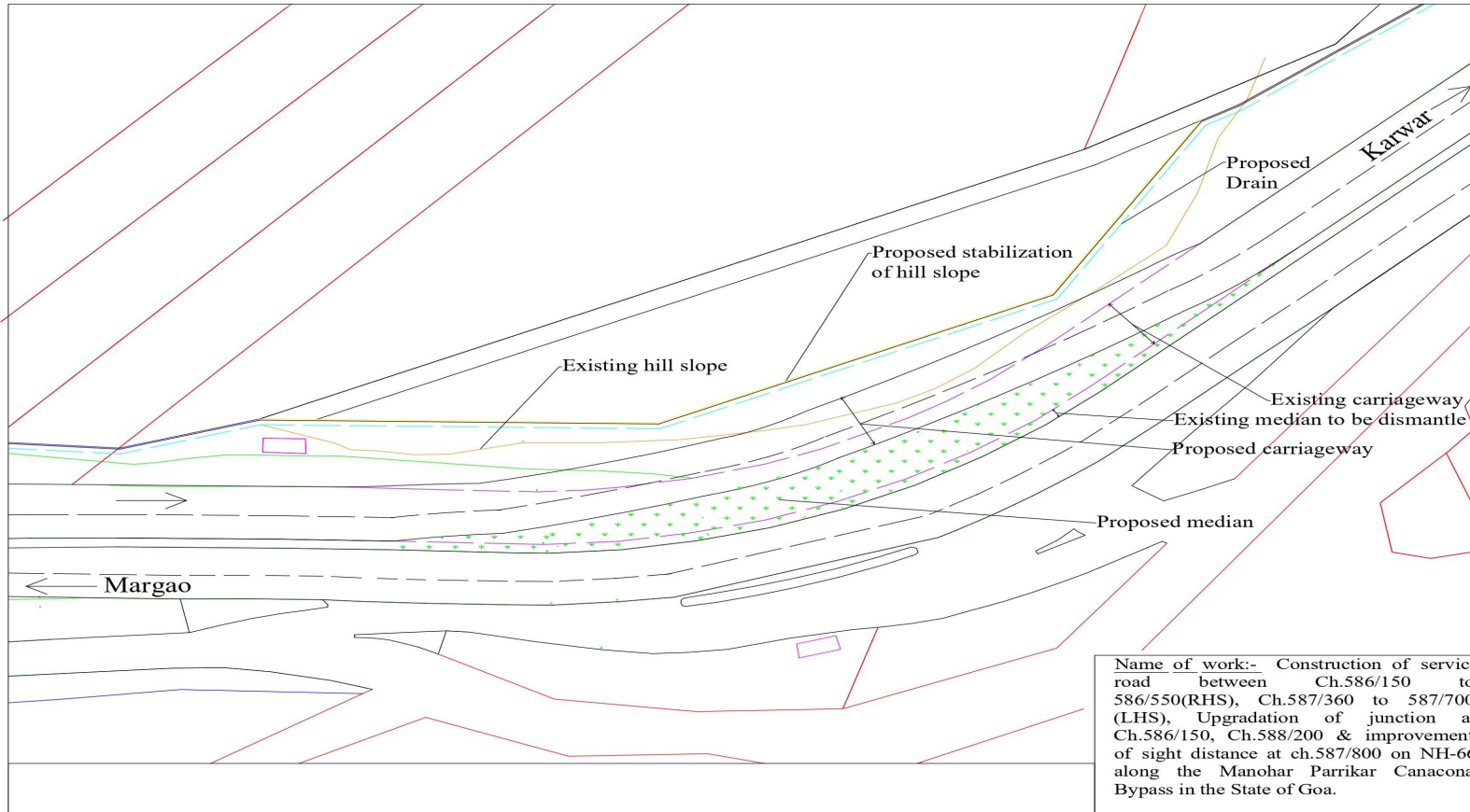
Improvement of curve at km.587.800 to km.587.900
