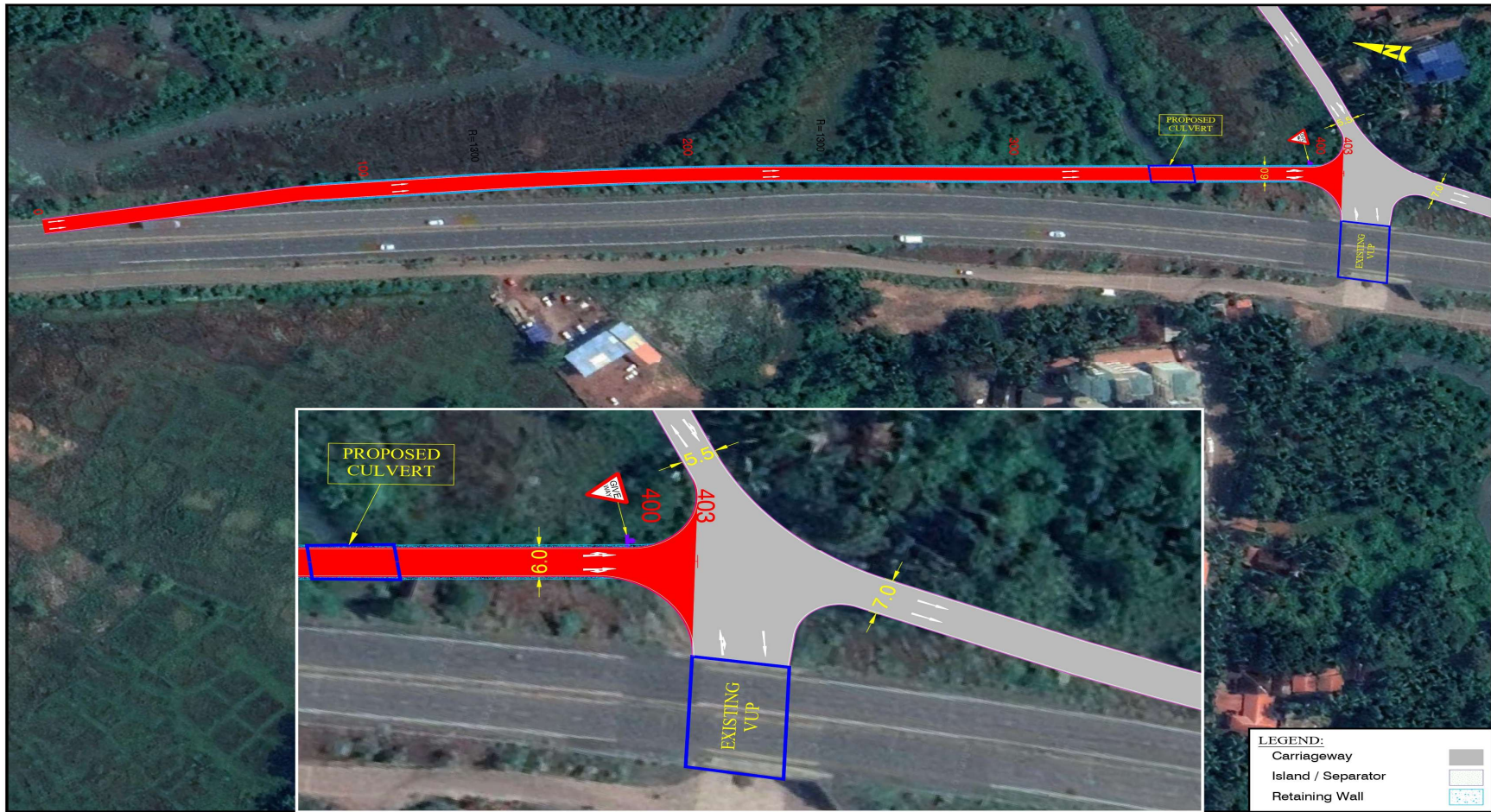
Junction Drawing - KM.587/700
