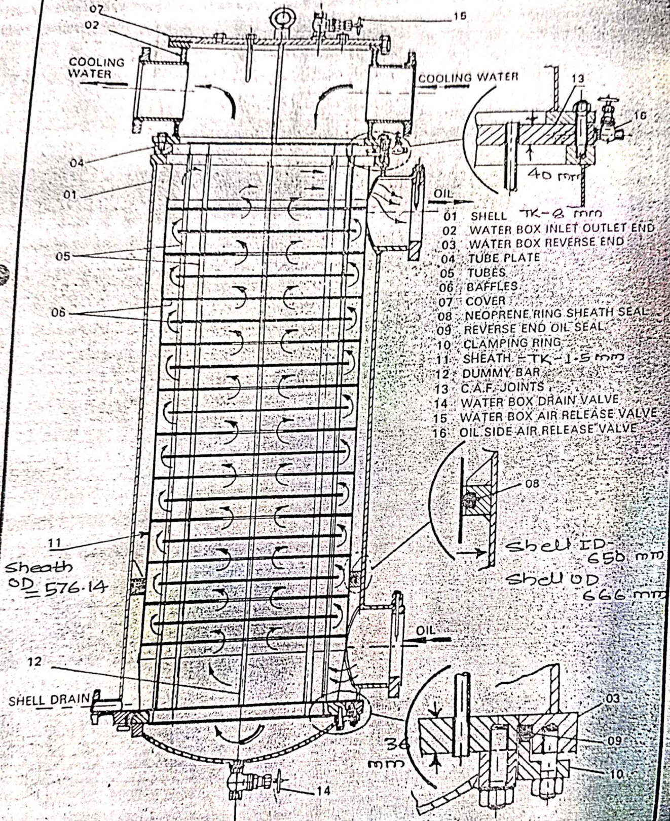
SECTIONAL VIEW OF OIL COOLER
