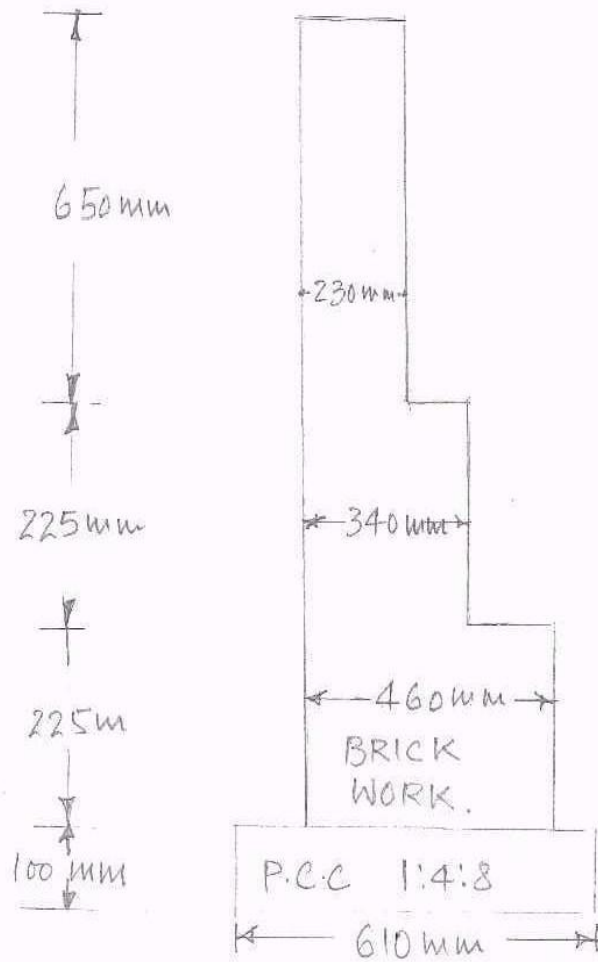
Figure 1 The Dimensions can Change as per the site conditions
