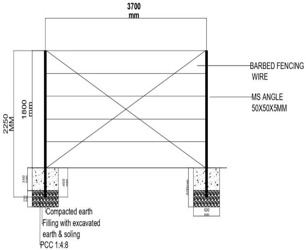
TYPICAL SECTION OF BARBED FENCING AT ANNEX LAND
