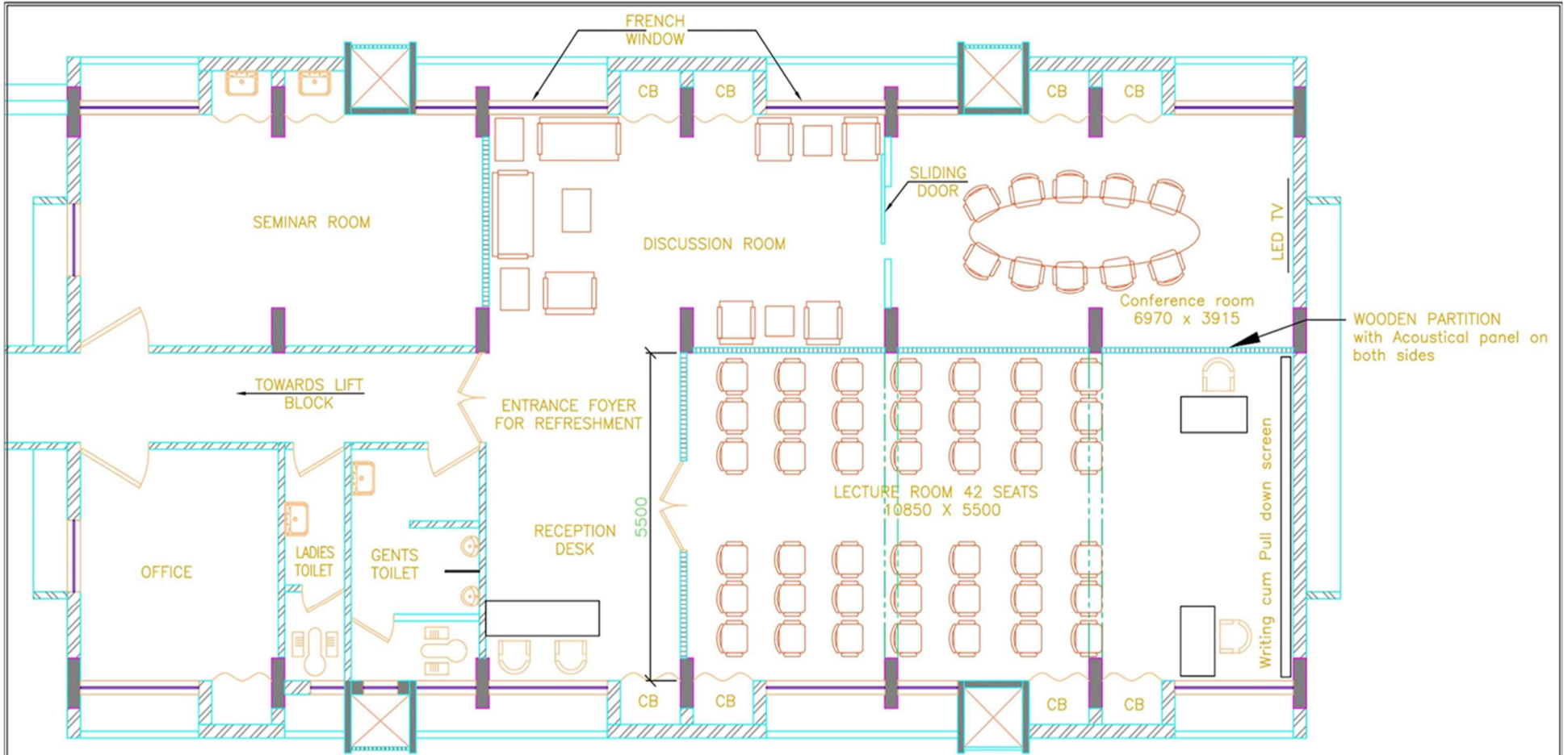
PROPOSAL FOR REMODIFICATION OF EXISTING SPACE INTO CONFERENCE ROOM AND LECTURE HALL IN FIRST FLOOR AT RAMANUJAN GUEST HOUSE TIFR, COLABA.
