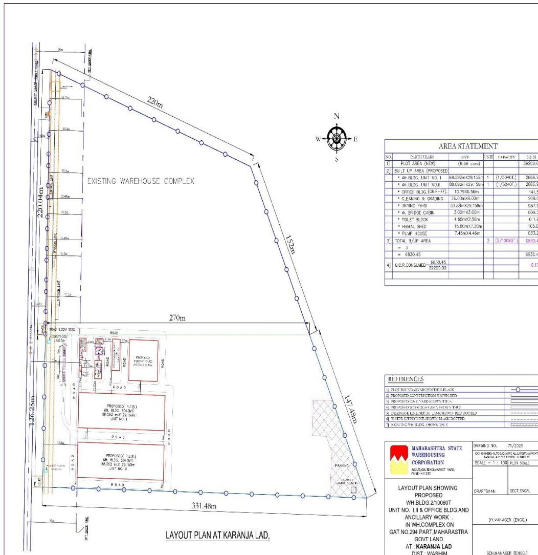
Dwg.1 Site Layout Plan
