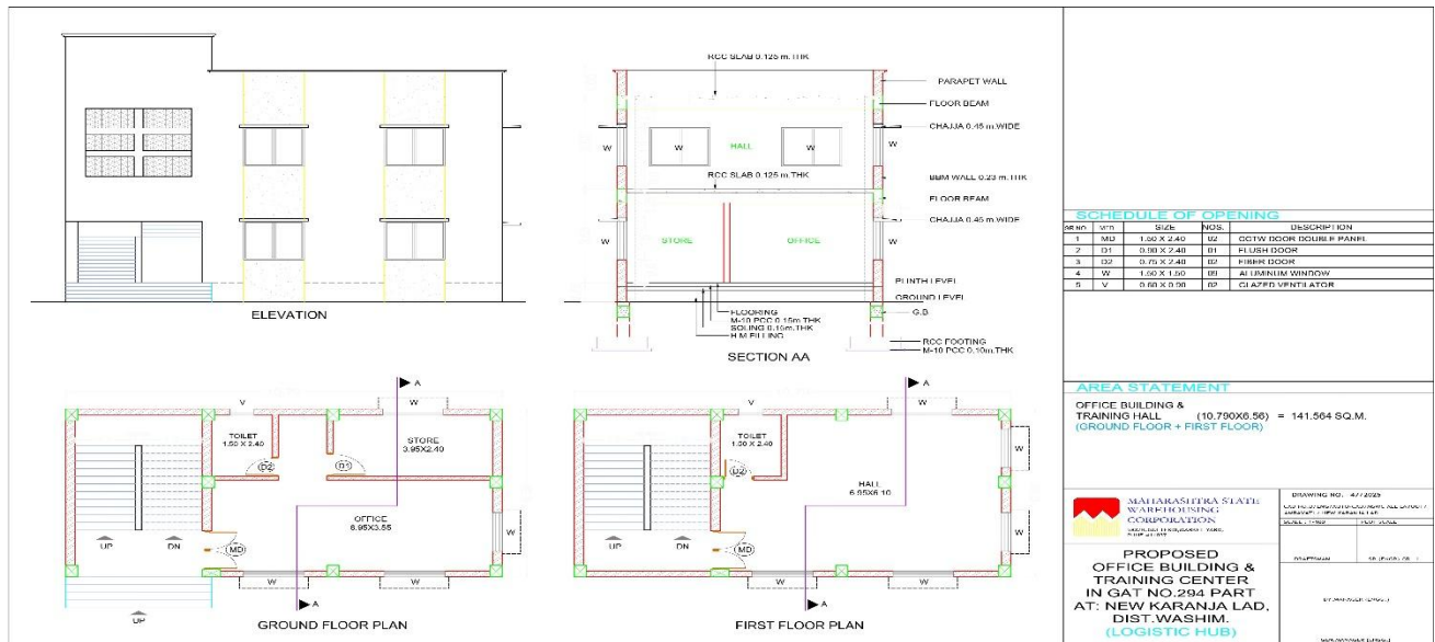
Dwg. 3 Office Building Plan, Section and Elevation
